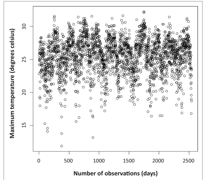
FIGURE 1: Plot of average maximum daily temperature (°C) for the period 2000–2010. Only data for the period September–April of each year are included.
